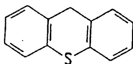
Thioxanthene
